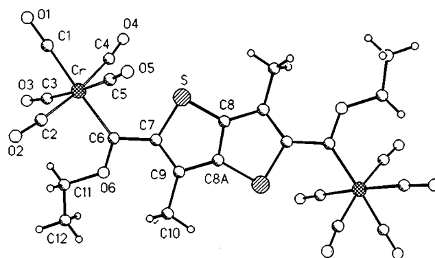
Figure 2. Molecular structure of complex 2 ; selected bond lengths [Å] and angles ^\circ : \text{Cr--C1} 2.068(3), \text{S--C4A} 1.721(2), \text{S--C2} 1.745(3), \text{C1--C2} 1.473(4), \text{C2--C3} 1.393(4), \text{C3--C4} 1.415(4), \text{C4A--C4} 1.378(5), \text{O6--C1--C2} 105.0(2), \text{O6--C1--Cr} 129.2(2), \text{C2--C1--Cr} 125.7(2)
